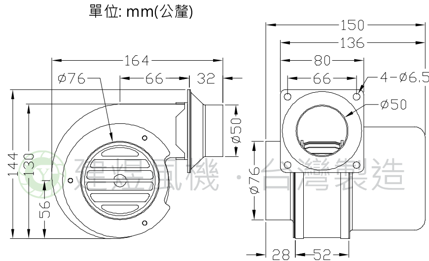
敞極馬達/Shaded pole motor
